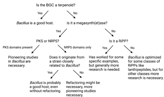
Fig. 3 Decision tree to verify whether Bacillus could be suitable for the expression of a given BGC.
