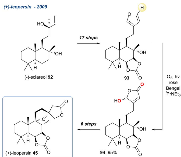
Scheme 11 Semi-synthesis of (+)-leopersin ( 45 ) from (–)-sclareol ( 92 ).
