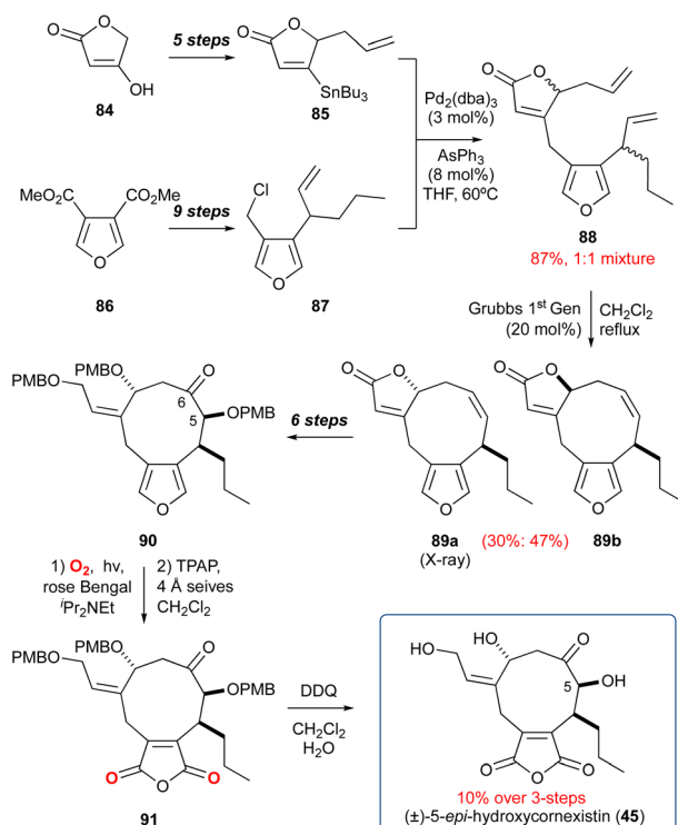
Scheme 10 Unveiling of the anhydride of the cornexistin's using a KDM/oxidation protocol.
