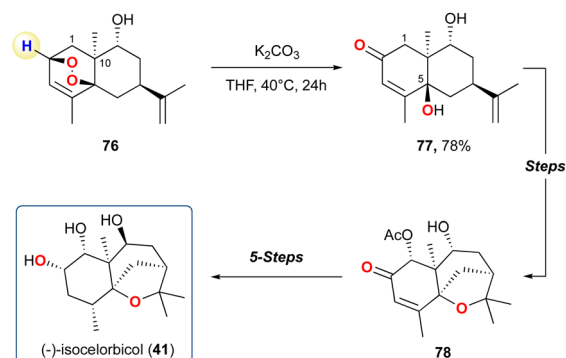
Scheme 7 Zhou et al. use of the KDM rearrangement to initially give precursor 77 which was subsequently used to give (-)-isocolorbicol 41 .
