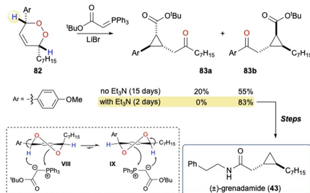
Scheme 9 The first synthesis of (±)-grenadamide using a phosphorus ylide mediated KDM cascade, with initial conditions providing two isomeric cyclopropanes 83a and 83b .
