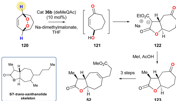
Scheme 18 Priest and co-workers use of the desymmetrisation of a prochiral endoperoxides to provide a rapid synthesis of the trans -xanthanolides skeleton.
