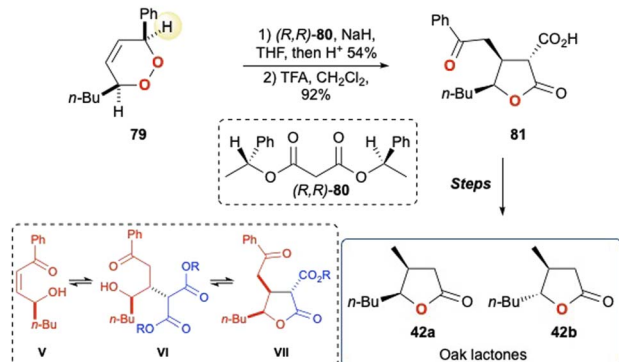
Scheme 8 The enantioselective total synthesis of oak lactones 42a and 42b , using a KDM rearrangement mediated by a chiral malonate with \gamma -lactonisation as a key step.
