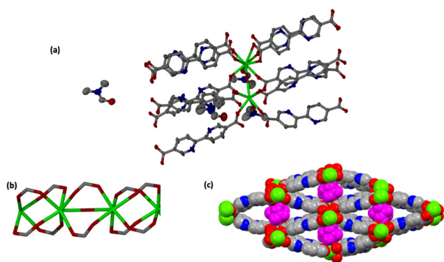
Fig. 2 (a) Coordination environment in JMS-11 showing the linker surrounding the metal centres. Hydrogens are omitted for clarity, and coordinated and uncoordinated DMF molecules are also shown. (b) Rod SBU and (c) packing diagram of JMS-11 viewed along the c -axis; the guest coordinated DMF molecules are shown in purple.
