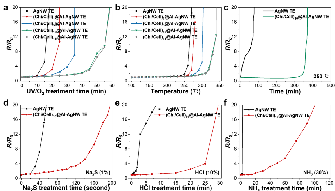
Fig. 3 Relative variation in the electrical resistance of AgNW, (\text{Chi}/\text{Cell})_1 , (\text{Chi}/\text{Cell})_5 , (\text{Chi}/\text{Cell})_{10} , and (\text{Chi}/\text{Cell})_{15} @Al-AgNW TEs as a function of (a) UV/O 3 treatment time and (b) temperature (100 to 350 °C at a ramping rate of 10 °C min −1 ). (c) Relative variation in the electrical resistance of AgNW and (\text{Chi}/\text{Cell})_{10} @Al-AgNW TEs at 250 °C as a function of time. Relative variation in the electrical resistance of AgNW and (\text{Chi}/\text{Cell})_{10} @Al-AgNW TEs as a function of time with treatments of (d) Na 2 S (1%), (e) HCl (10%), and (f) NH 3 (30%) solutions.
