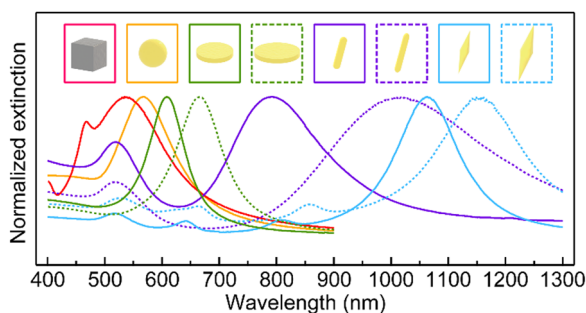
Fig. 4 Representative extinction spectra for Ag NCs (73 nm in edge length, solid pink line), Au NSs (88 nm in diameter, solid yellow line), circular Au NPLs (79 nm in diameter, 22 nm in thickness, solid green line); 99 nm in diameter, 22 nm in thickness, dotted green line), Au NRs (14 nm in diameter, 59 nm in length, solid purple line; 10 nm in diameter, 63 nm in length, dotted purple line), Au NBPs (59 nm in waist diameter, 230 nm in length, solid blue line; 70 nm in waist diameter, 276 nm in length, dotted blue line). All samples are dispersed in aqueous solutions for extinction measurements. The data of Au NSs, Au NPLs and Au NBPs are reproduced from ref. 146, 155, 157 with permission from Wiley-VCH publisher, Copyright 2014, 2018 and 2015, respectively. The data of Au NRs are reproduced from ref. 158 with permission from ACS publisher, Copyright 2006.
