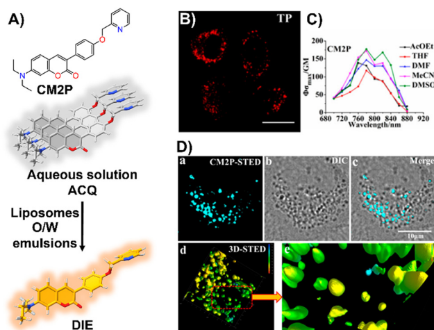
Fig. 19 (A) Chemical structure of CM2P and its DIE mechanism mediated by liposomes or oil/water emulsions. (B) and (C) Two-photon fluorescence imaging of HeLa cells stained with CM2P (B) and the two-photon molecular brightness of CM2P across various solvents (C). (D) Morphological characterization of LDs in live HeLa cells stained with CM2P : (a) STED image, (b) bright-field image, (c) merged image of (a) and (b), (d) 3D-STED image, and (e) zoomed-in view of (d). Rainbow calibration bar, Z-scale (0–10 \mu\text{m} ); scale bar: 10 \mu\text{m} . Reprinted with permission from ref. 29. Copyright 2019 American Chemical Society.
