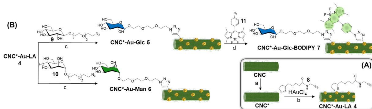
Scheme 1 (A) Synthesis of CNC*-Au-LA 4 . Reaction conditions: a. Sulfur trioxide pyridinium complex, dimethyl sulfoxide, 4 h, 25 °C; b. \text{HAuCl}_4 , \text{NaBH}_4 , water:methanol (1 : 9), and 8 . (B) Synthesis of CNC*-Au-Glc 5 , CNC*-Au-Man 6 , and CNC*-Au-Glc-BODIPY 7 . Reaction conditions for c and d: \text{CuSO}_4 , sodium ascorbate (water for c and DMF for d), overnight, room temperature.
