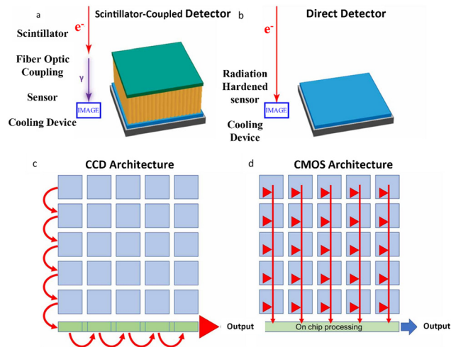
Fig. 4 The difference between conventional CCDs and DEDs. (a) The electron-photon-sensor process in CCDs. (b) The electron-sensor process in DEDs. (c) The row-by-row readout architecture in CCDs. (d) The simultaneous readout architecture in every pixel in DEDs. Reproduced with permission. 28 Copyright 2020, American Chemical Society.
