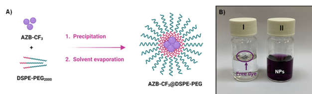
Fig. 3 (A) Scheme showing the preparation of \text{AZB-CF}_3 @DSPE-PEG NPs, (B) vials containing free dye \text{AZB-CF}_3 (I) and \text{AZB-CF}_3 @DSPE-PEG NPs (II) suspended in PBS.
