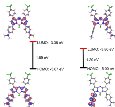
Fig. 2 Optimized structures and frontier molecular orbitals (HOMO and LUMO) plotted at an electron density value of 0.035 of \text{AZB-CF}_3 in ground states (left) and excited states (right) and their corresponding energy gaps ( \Delta E in eV) computed at the B3LYP/6-311G level of theory.
