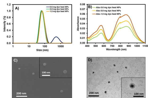
Fig. 4 (A) Dynamic light scattering (DLS): the intensity-based size distribution of \text{AZB-CF}_3 @DSPE-PEG NPs with 0.6 mg, 0.8 mg, and 1.0 mg of dye feed. (B) Absorption spectra of \text{AZB-CF}_3 @DSPE-PEG NPs with different amounts of dye feed. (C) Scanning electron microscope (SEM) images and (D) transmission electron microscope (TEM) images of \text{AZB-CF}_3 @DSPE-PEG NPs with 1.0 mg dye feed.
