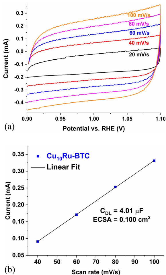
Fig. 7 (a) CV plots of \text{Cu}_{10}\text{Ru-BTC} with different scan rates used for the calculation of the ECSA; (b) current vs. scan rate plot obtained from the CVs in (a) ( C_{\text{DL}} = double layer capacitance, ECSA = electrochemical surface area).
