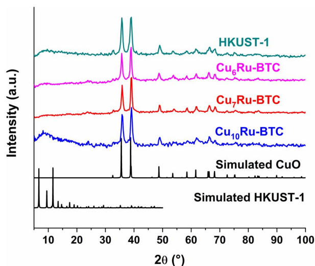
Fig. 8 PXRD patterns of mechanochemically synthesized HKUST-1, \text{Cu}_6\text{Ru-BTC} , \text{Cu}_7\text{Ru-BTC} , \text{Cu}_{10}\text{Ru-BTC} , following 24 h in 1 \text{ mol L}^{-1} KOH solution, simulated CuO (COD: 15-26990) and simulated HKUST-1 (CCDC no. 112954).
