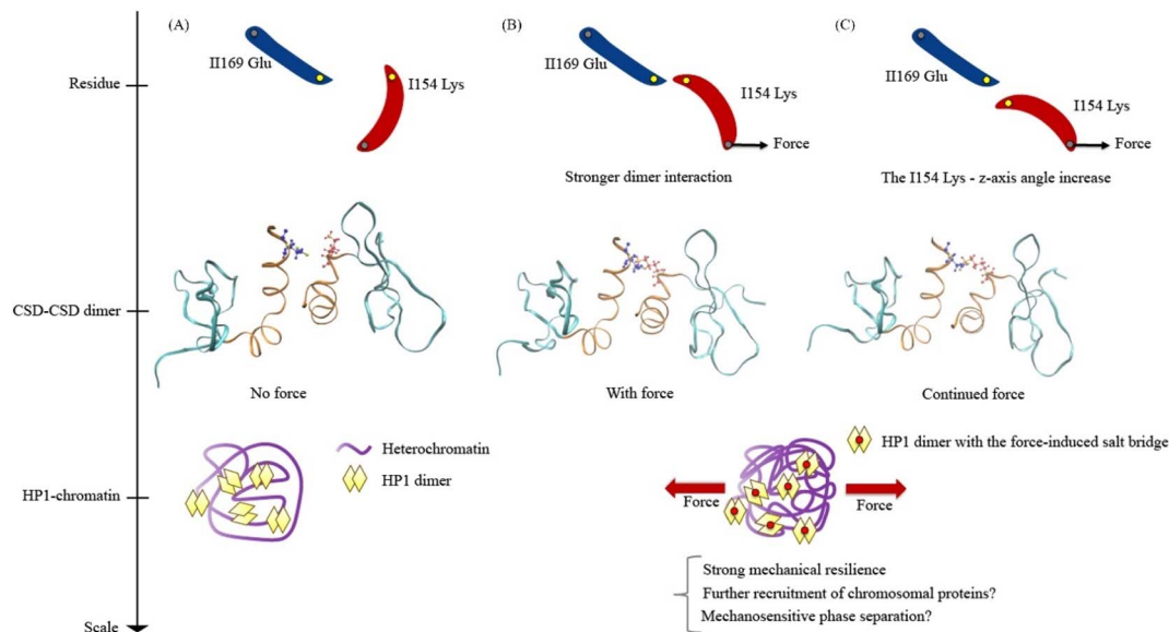
Fig. 8 Models of HP1 \alpha mechanical response at residue, the CSD–CSD dimer, and HP1 \alpha –chromatin scales, presented from top to bottom: (A) no-force condition: the ^1\text{Lys154} – ^{12}\text{Glu169} salt bridge interaction is less likely to occur, resulting in low mechanical resilience for HP1. (B) Force condition: under applied force, the ^1\text{Lys154} angle changes, leading to the development of the ^1\text{Lys154} – ^{12}\text{Glu169} salt bridge interaction. This strengthens the interaction within the CSD–CSD dimer, enhancing the mechanical resilience of HP1 \alpha . (C) Dissociation processes: continuous external force disrupts the ^1\text{Lys154} – ^{12}\text{Glu169} salt bridge interaction by increasing the ^1\text{Lys154} angle against the applied force direction. Consequently, high mechanical resilience is compromised.
