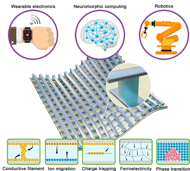
Fig. 1 Applications and mechanisms of flexible memristors.
