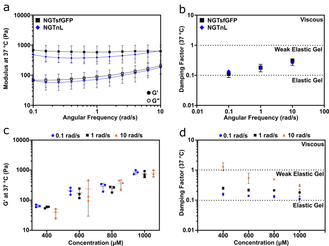
Fig. 2 NGT-fusion proteins form concentration dependent, weak elastic gels. (a) G' (closed circles) and G'' (open circles) of NGTsfgf and NGTnL gels at 37 °C from 10 to 0.1 \text{rad s}^{-1} . (b) Damping factor ( G''/G' ) of NGTsfgf and NGTnL. (c) G' of NGTsfgf gels at varying concentrations at angular frequencies of 0.1, 1, and 10 \text{rad s}^{-1} . (d) Damping factor ( G''/G' ) of NGTsfgf gels at varying concentrations and angular frequencies of 0.1, 1, and 10 \text{rad s}^{-1} . Measurements taken at a strain of 0.3%.
