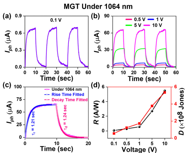
Fig. 7 MGT: transient ( I - t ) photo response curve at (a) 0.1 V and (b) 0.5–10 V, (c) fitted time response curve, and (d) responsivity and detectivity versus voltage graph of MGT under 1064 nm illumination.
