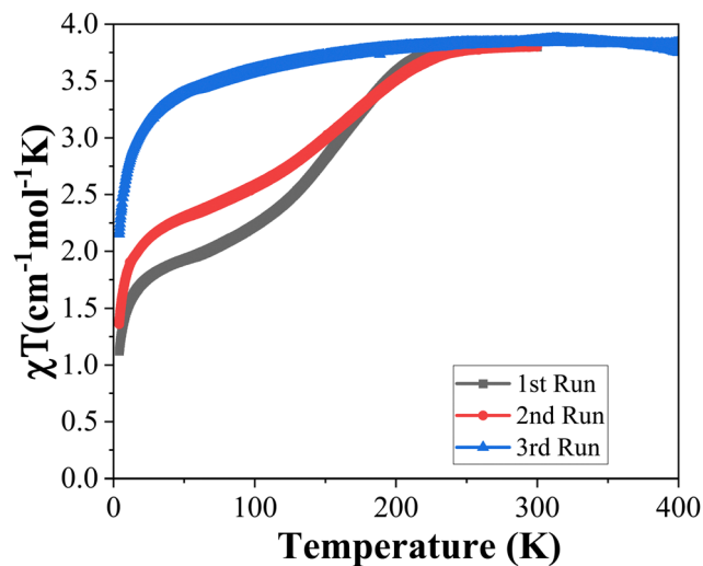
Fig. 6 \chi^2 vs. T of 1 for three consecutive runs.
