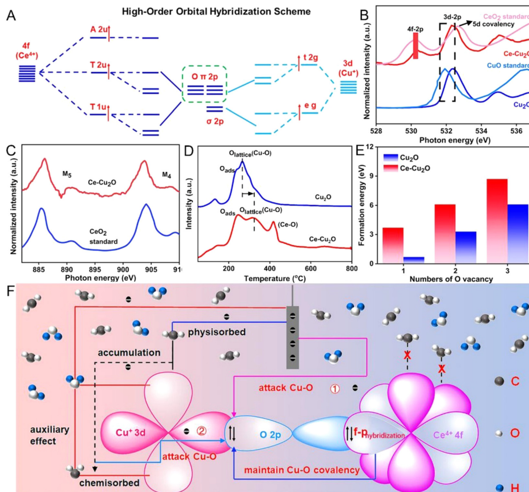
Fig. 4 Molecular orbital representation of \text{Ce}^{4+} 4f O 2p \text{Cu}^{+} 3d coupling (A). Ex situ xXAS measurements of the O-K edge in \text{CeCu}_2\text{O} and \text{Cu}_2\text{O} catalysts (B). Ex situ xXAS at the Ce-M4,5 edge in \text{Ce-Cu}_2\text{O} (C). \text{Ce-Cu}_2\text{O} and \text{Cu}_2\text{O} \text{O}_2 -TPD spectra (D). Formation Energy requirements for OVs in \text{Ce-Cu}_2\text{O} and \text{Cu}_2\text{O} , is presented in (E). (F) A schematic showing how the connection between the high-order orbitals 4f and 2p in \text{Ce-Cu}_2\text{O} prevents \text{CuO} deactivation and shields the \text{Cu}^{+} site from electron attack during the \text{CO}_2\text{RR} . Reproduced with permission from ref. 47. Copyright 2023, American Chemical Society.
