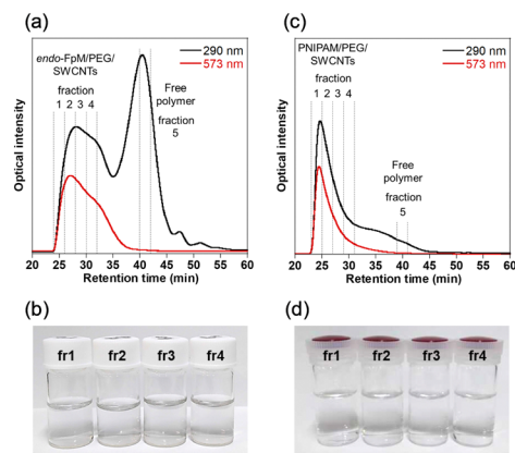
Fig. 2 (a), (c) SEC chromatograms and (b), (d) photographs of fractionated solutions of (a), (b) endo -FpM/PEG/SWCNTs and (c), (d) PNIPAM/PEG/SWCNTs.
