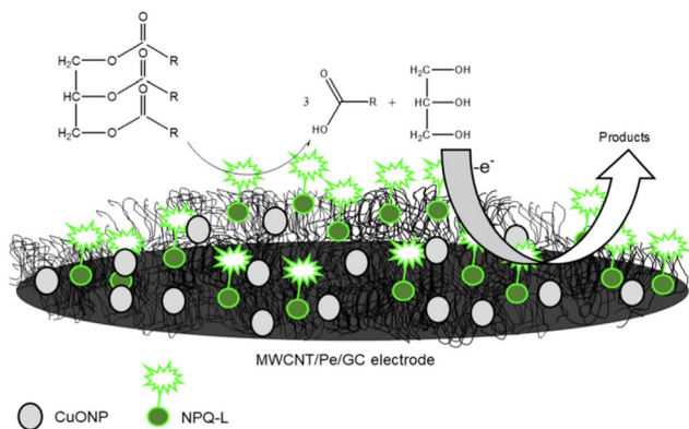
Fig. 16 Schematic representation of glycerol determination using copper oxide/multiwalled carbon nanotube/pectin/GCE (reprinted from ref. 179 with permission from Elsevier).
