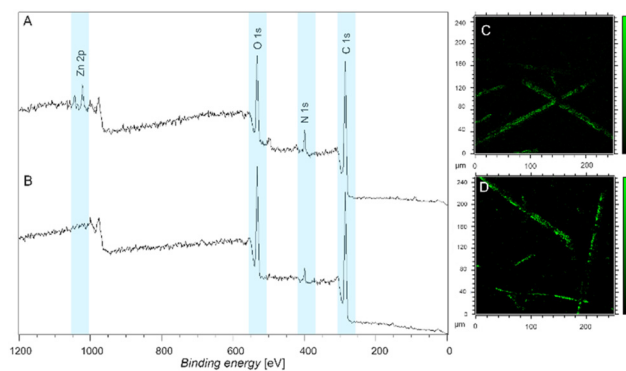
Fig. 6 (A) XPS wide scan spectra of fibers coated with ligand-modified L-DOPA (7), exposed to \text{Zn}^{2+} solution; (B) corresponding XPS wide scan spectra of pristine fibers exposed to \text{Zn}^{2+} solution; (C) and (D) display the ToF-SIMS spatially resolved mapping of \text{Zn}^{2+} . The images clearly demonstrate the presence of coordinated metal on the fibers. Intensity variations seen on the fibers are due to the non-uniform size of the fibers.
