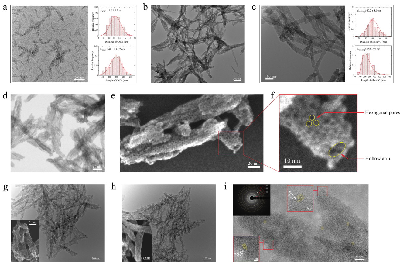
Fig. 2 Electron microscopic studies of CNCs, SilicaNQs, and SiNQs; (a) needle-like CNC particles with an average length of 144 nm and width of 12.5 nm, (b) porcupine quill-like silicate gel product from sol-gel reaction, (c) SilicaNQ particles from calcination process showing average length of 252 nm and width of 40.2 nm, (d) BF S-TEM image of SilicaNQs reveals the hollow tunnels within 1D silica arms, (e) ultrahigh porous surface of SilicaNQs with an ordered arrangement of hexagonal pores, (f) a single SilicaNQ arm possessing hexagonal surface pores and a central hollow core, (g) TEM and S-TEM micrographs of SiNQ-a, (h) TEM and S-TEM micrographs of SiNQ-g, and (i) high-resolution TEM micrograph of SiNQ arms, revealing crystalline pockets distributed in an amorphous matrix. Electron diffraction patterns show the presence of major crystal systems of elemental Si in the structure of SiNQ material.
