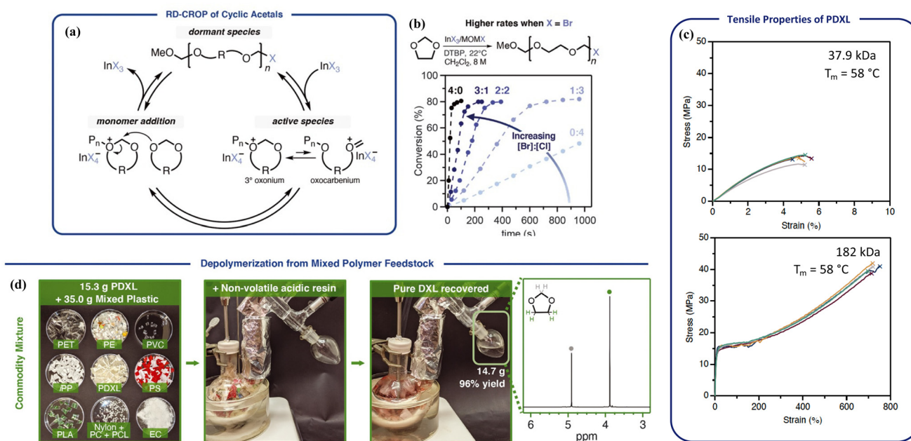
Fig. 9 Poly(1,3-dioxolane) (PDXL) circular system ( T_c = 13^\circ\text{C} ). (a) Proposed mechanism for the reversible-deactivation polymerization of cyclic acetals. (b) Reaction rate increases when increasing the [\text{Br}]:[\text{Cl}] ratio in \text{InX}_3/\text{MOMX} catalyst/initiator system. (c) Tensile properties of PDXL with molecular weight of 37.9\text{ kg mol}^{-1} (top) and 182\text{ kg mol}^{-1} (bottom). (d) Recovery of the monomer from a mixed commodity plastics feedstock. Recycling condition: PDXL 80\text{--}180\text{ kg mol}^{-1} , acid resin (Dowex-50, 5 wt%, nonvolatile), mechanically stirred at 150 \pm 5^\circ\text{C} , distilled under ambient pressure, monomer recovered in 96% yield and >99% purity. Reproduced from ref. 109 with permission from AAAS, copyright 2021.
