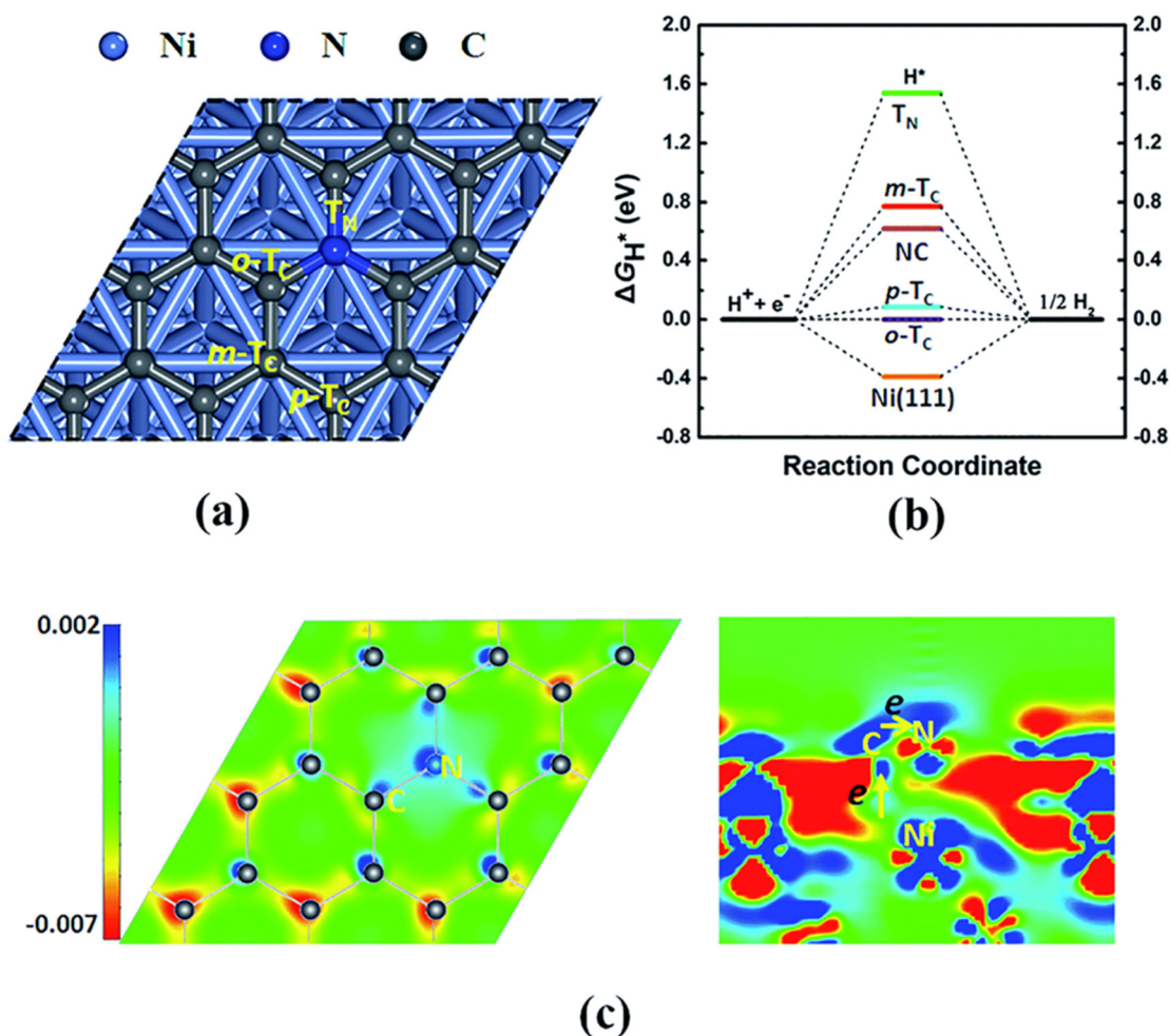
Fig. 28 Typical electron transfer process Ni \rightarrow C \rightarrow N. (a) Theoretical model used in DFT calculations and obtained adsorption site of H + on model surface. (b) Computed free energies for adsorption sites. (c) Charge density difference of the Ni(111)@NC model, where red and blue areas signify low and high electron density, respectively. Reprinted with permission from ref. 239. Copyright 2020, The Royal Society of Chemistry.
