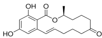
Alternariol monomethyl ether
