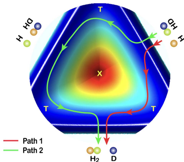
Fig. 2 A cut view through the \text{H} + \text{HD} potential energy surface with transition states (T) and conical interaction (X). Two representative reaction pathways are shown: a one-transition-state reaction path (Path 1) and a two-transition-states reaction path (Path 2). Adapted from ref. 175 and used with permission under lic. no. 5744150372346.
