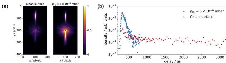
Fig. 7 (a) Comparison of the CO scattering VMI on the clean surface (no oxygen in the chamber) and p_{\text{O}_2} = 5 \times 10^{-6} mbar at T_s = 600 K. (b) shows the corresponding CO scattering kinetic trace in (a); data are selected within a 20-degree sector below the center and signals are normalized to the incident beam intensity.
