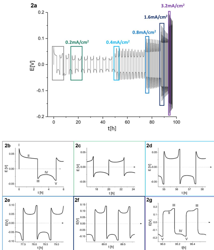
Fig. 2 (a) Voltage trace ( E vs. t ) of successive galvanostatic cycling of a total of 1 mA h cm -2 of Li at increasing currents of 0.2, 0.4, 0.8, 1.6 and 3.2 mA cm -2 in lithium symmetric cell with 1 M LiPF 6 in EC : DMC (LP30). (b)–(g) Magnification of selected voltage traces ( E vs. t ) of successive galvanostatic cycling of a total of 1 mA h cm -2 of Li at increasing currents of (b) 0.2, (c) 0.2, (d) 0.4, (e) 0.8, (f) 1.6 and (g) 3.2 mA cm -2 in lithium symmetric cell with 1 M LiPF 6 in EC : DMC. For 0.2 mA cm -2 both the first (b) and the fourth (c) cycles are presented. Characteristic peaks and processes are labelled, following the assignments made by Dasgupta et al. 1,2
