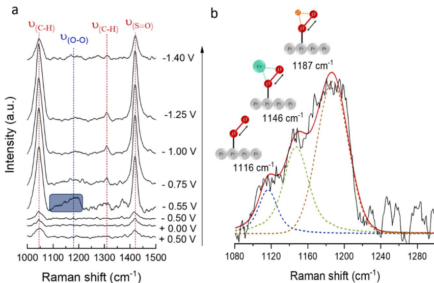
Fig. 7 (a) Potential-dependent in situ SHINERS spectra obtained from a Pt(111) electrode in a solution containing 0.1 M \text{CsClO}_4 /DMSO, purged with Ar and, subsequently, saturated with \text{O}_2 . (b) Voigt model fitting of \nu_{(\text{O}-\text{O})} at -0.55 \text{ V} .
