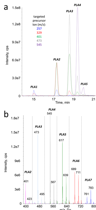
Fig. 4 a) Precursor ion scan analysis of aged PLA with positive electrospray ionization. The targeted ions were those identified by MS2 analyses and are listed on the figure; b) neutral loss analysis of aged PLA with positive electrospray ionization. The monitored loss was -72 . The figure shows the m/z ratio of the pseudo-molecular ions detected under each chromatographic peak.
