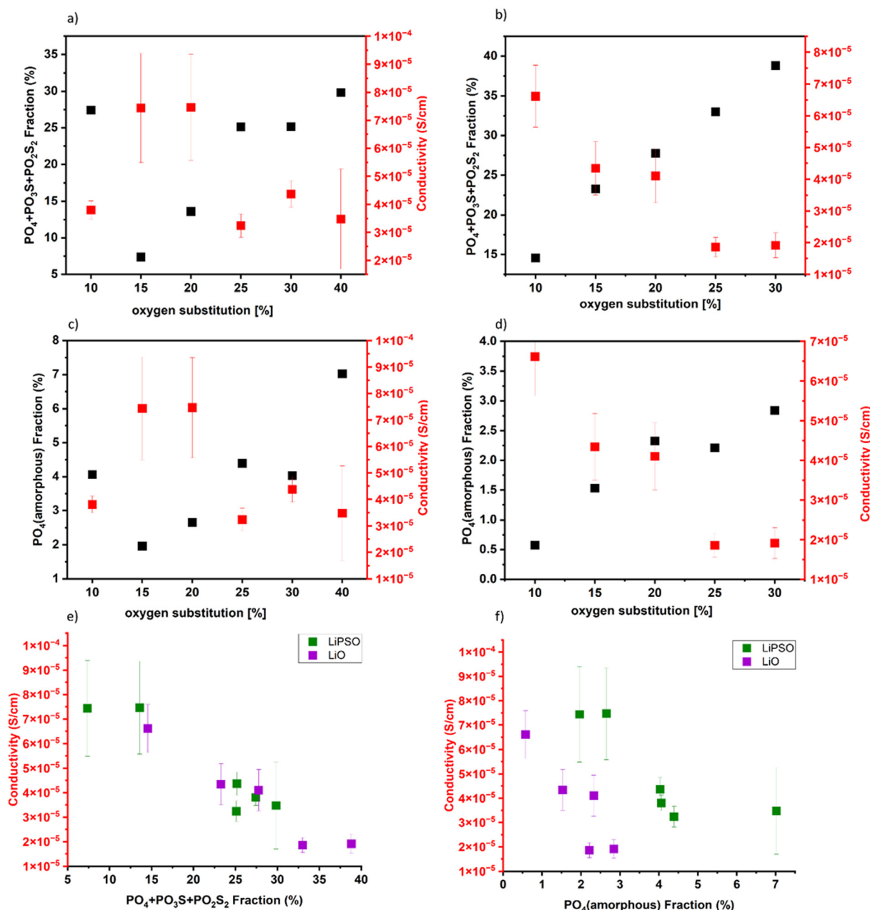
Fig. 7 (a and b) combined fraction of all tetrahedra with n_O > 2 (black) and corresponding Li-ion conductivity (red) vs. total oxygen substitution of LIPSO (a) and LIO (b). (c and d) Amorphous \text{PO}_4 fraction and Li-ion conductivity vs. total oxygen substitution of LIPSO (c) and LIO (d). (e and f) Li-ion conductivity vs. fraction of all tetrahedra with n_O > 2 (e) and amorphous \text{PO}_4 fraction (f) across all samples from both LIPSO (green) and LIO (purple) samples.
