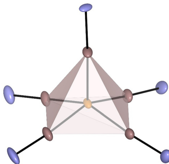
Fig. 1 Left: molecular structure of [Ru(\text{GaTMP})_5] ( 1 ) in the solid state determined by single crystal X-ray diffraction. Ru: yellow, Ga: pink, N: blue and C: grey. Hydrogen atoms and disordered molecule fragments are omitted. C and N are displayed as wireframe. Right: square pyramidal coordination polyhedron calculated from crystal structure data. Thermal ellipsoids are shown at the 50% probability level. Selected bond lengths [Å] and angles [°]: Ru1–Ga3: 2.274(10) Ru1–Ga2 #1 /Ga2: 2.281(7), Ru1–Ga1 #1 /Ga1: 2.291(6), Ga3–Ru1–Ga2 #1 /Ga2: 104.6(2), Ga3–Ru1–Ga1 #1 /Ga1: 103.0(2), Ga2–Ru1–Ga1: 84.2(3), Ga2–Ru1–Ga1 #1 : 89.3(2). Note: Ga1/Ga1 #1 and Ga2/Ga2 #1 are symmetry related.
