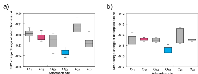
Fig. 4 Box plot of NBO charge change on the adsorption site by protonation in (a) \beta - XMo_{12} and (b) \beta - XW_{12} . The upper and lower whiskers, respectively, represent the maximum and minimum values. Magenta, sky-blue, and grey boxes represent the change in NBO charge on O_{12} , O_{22e} , and other adsorption sites, respectively.
