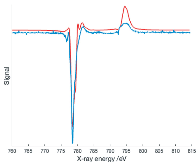
Fig. 6 XMCD spectrum of [\text{Co}(\text{dipyvd})_2]^{2+}(\text{PF}_6)_2 at 2 K/6T (blue) along with crystal field multiplet simulation (red line) – simulation parameters 10Dq = 2.0 eV, Slater–Condon integrals scaled by a factor of 0.69.
