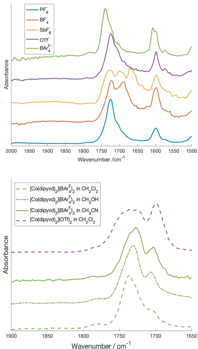
Fig. 1 Top: carbonyl region of the IR spectrum of crystalline [\text{Co}(\text{dipyvd})_2]^{2+} salts. Bottom: carbonyl region of [\text{Co}(\text{dipyvd})_2](\text{BARF}_4)_2 and [\text{Co}(\text{dipyvd})_2]^{2+}(\text{OTf})_2 in solution.
