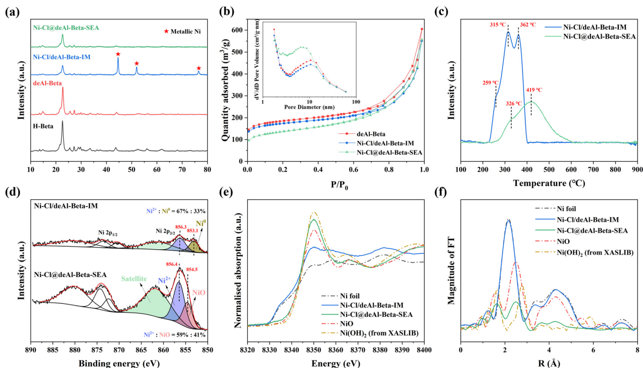
Fig. 2 (a) XRD patterns and (b) N_2 physisorption isotherms of the beta zeolite supports and the associated Ni catalysts; (c) H_2 -TPR (of the as-prepared Ni catalysts after drying at 120^\circ C for 4 h), (d) XPS profiles, (e) XANES and (f) Fourier transform of k^3 -weighted EXAFS spectra of the reduced Ni-Cl@deAl-beta-SEA and Ni-Cl/deAl-beta-IM. Note that the data of Ni(OH)_2 is referred to the XASLIB database.
