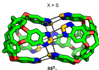
Fig. 17 Halogen- and chalcogen-bond interactions, including with halonium ions, can be used to assemble both homo- and heteromeric capsules. R groups omitted from SCXRD structures for clarity.
