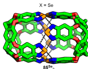
Fig. 17 Halogen- and chalcogen-bond interactions, including with halonium ions, can be used to assemble both homo- and heteromeric capsules. R groups omitted from SCXRD structures for clarity.
