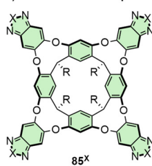
Fig. 17 Halogen- and chalcogen-bond interactions, including with halonium ions, can be used to assemble both homo- and heteromeric capsules. R groups omitted from SCXRD structures for clarity.
