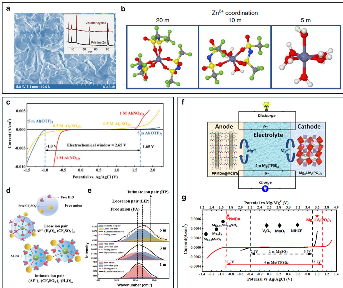
Fig. 21 Water-in-salt electrolytes. (a) SEM image and XRD pattern (inset) of a Zn anode cycled in the HCZE. (b) \text{Zn}^{2+} -solvation structures in the electrolytes with 1 m \text{Zn}(\text{TFSI})_2 + \text{LiTFSI} of 5 m, 10 m and 20 m, respectively. Reproduced with permission from ref. 372 Copyright 2018, Springer Nature. (c) The linear sweep voltammetry in the Al-WISE electrolyte in comparison to 1 M \text{Al}(\text{NO}_3)_3 and 0.5 M \text{Al}_2(\text{SO}_4)_3 electrolytes. (d) Schematic diagram of the \text{Al}^{3+} -solvation structures showing the free anion (FA), loose ion pair (LIP) and intimate ion pair (IIP). (e) Raman spectra of 1, 3, and 5 M \text{Al}(\text{OTf})_3 . Reproduced with permission from ref. 378 Copyright 2019, American Chemical Society. (f) Schematic illustration of Mn-ion batteries with the electrolyte of 4 m \text{Mg}(\text{TFSI})_2 . (g) Electrochemical stability window of the 4 m \text{Mg}(\text{TFSI})_2 aqueous electrolyte. Reproduced with permission from ref. 379 Copyright 2017, American Chemical Society.
