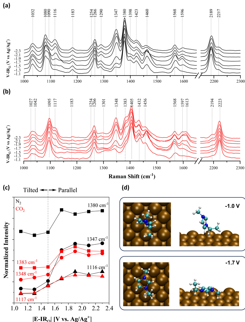
Fig. 13 Potential dependent SERS spectra of [EMIM][2-CNpyr] under (a) N 2 and (b) CO 2 , (c) SERS peak intensity as a function of absolute applied potential (E-IR 0 ). The dotted line marks the potential of the change in the orientation of imidazolium species under N 2 (black) and CO 2 (red). Peaks: 1116 cm -1 (triangles) for \delta(\text{C}_4\text{C}_5\text{-H}) ; 1347 cm -1 for \nu(\text{Im-ring}) + \nu(\text{CH}_2(\text{N})) (circle); 1380 cm -1 for \nu(\text{Im-ring}) + \nu(\text{CH}_2(\text{N})) + \nu(\text{CH}_3) (square). (d) Lowest energy geometries calculated for [EMIM] + at -1.0 and -1.7 V on Cu(100) (top and side views) indicating the preference of the parallel orientation at a more negative potential. Atom color code: blue = N; cyan = C; white = H. Reprinted with permission from ref. 451. Copyright 2023, John Wiley and Sons.
