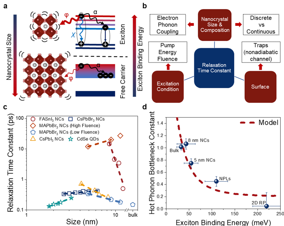
Fig. 8 Effect of perovskite nanocrystal size on the relaxation kinetics. (a) Schematic diagram to illustrate the relaxation pathway in a strongly-confined (excitonic) system vs. in a weakly-confined (free-carriers) system. The \alpha , \phi , and \chi are the hot-cold carrier, carrier-phonon, and hot exciton cooling coefficients, respectively. (b) Scheme of the factors that could influence the final relaxation time constant, i.e. , the time it takes for the hot carriers to relax to the band edge with the carrier temperature matching the surrounding lattice temperature. (c) Comparison of reports showing the influence of QD size on the relaxation time constant. The data included in panel c is from ref. 16 (CsPbBr 3 NCs), 114 (FASnI 3 NCs), 115 and 116 (MAPbBr 3 NCs), 117 (CsPbI 3 NCs), and 118 (CdSe QDs). (d) Hot phonon bottleneck parameters ( \beta ) for all CsPbBr 3 systems with different sizes and exciton binding energies, compared to a 2D (PEA) 2 PbI 4 thin film. A larger \beta value implies a more pronounced hot phonon bottleneck and slow hot carrier relaxation. Error bars correspond to a 99% confidence interval. The black dotted curve is the hot phonon bottleneck behavior as a function of E_b predicted by the kinetic model described in the main text. Panels a and b are inspired by ref. 113.
