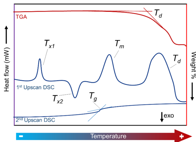
Fig. 13 DSC depiction (Heat flow vs. Temperature) and thermogravimetric analysis of a meltable crystalline MOF. TGA is represented as a red line showing a weight loss upon heating, indicating the decomposition temperature ( T_d ). DSC 1st and 2nd upscans are depicted in the graph as blue curves. 1st upscan shows multiple processes upon heating. Firstly, an endothermic recrystallisation (structural phase transition) denoted as T_{x1} . The second feature shows an exothermic phase transition ( T_{x2} ). Melting and decomposition processes also appear as endothermic features. A T_g appears in the 2nd DSC upscan of a crystalline MOF, after the material melted and formed a glassy phase during heating in the 1st upscan.
