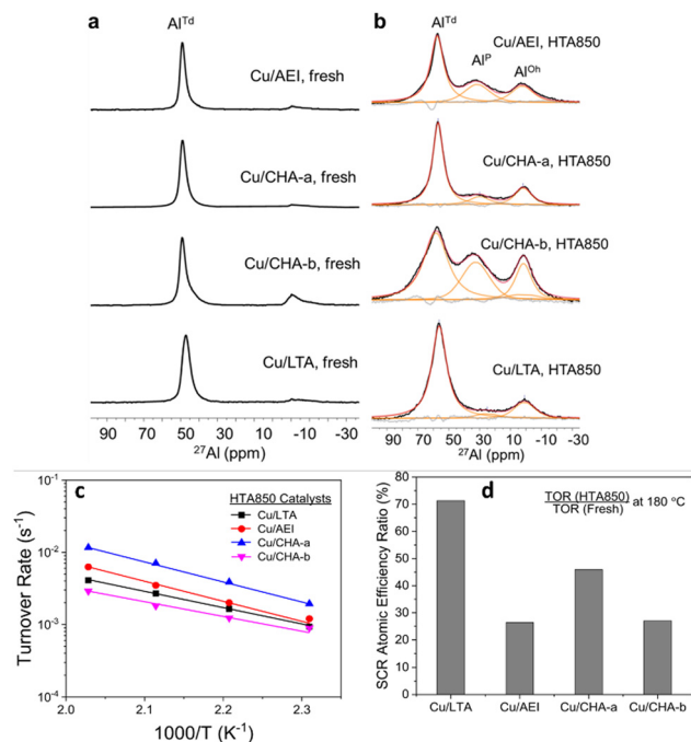
Fig. 22 (a) Spectra of fresh (a) and hydrothermally aged (b) Cu-zeolites. Arrange the turnover rates (TORs) as Arrhenius plots (c), and illustrate turnover rate (TOR) ratios at 180 °C between freshly prepared catalysts and (d) those subjected to hydrothermal ageing. Reproduced from ref. 326 with permission from Springer Nature, copyright 2023.
