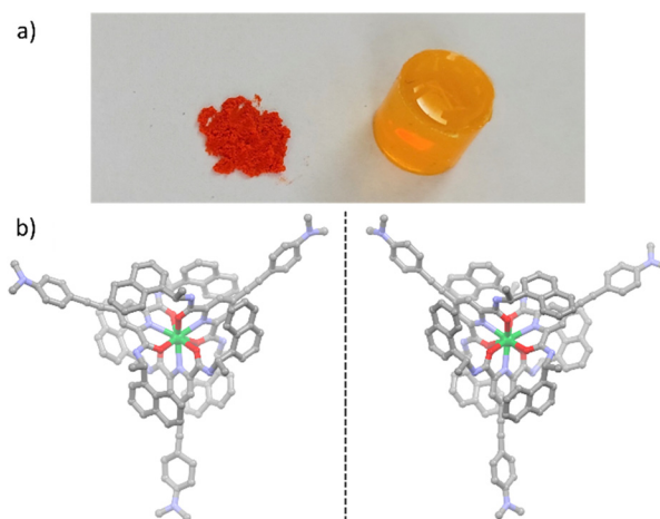
Fig. 1 (a) Pure powder of Yb(III) complex, on the left, and solution in PDMS polymer, on the right; (b) X-ray structures of [Yb( S,S -L NHHex2 ) 3 (OTf) 3 ]/ \Delta -Yb (left) and [Yb( R,R -L NHHex2 ) 3 (OTf) 3 ]/ \Lambda -Yb (right). Hexyl chains are simplified; hydrogen atoms, solvent molecules and OTf-anions are omitted for clarity. Green, Yb; red, O; blue, N and grey, C.
