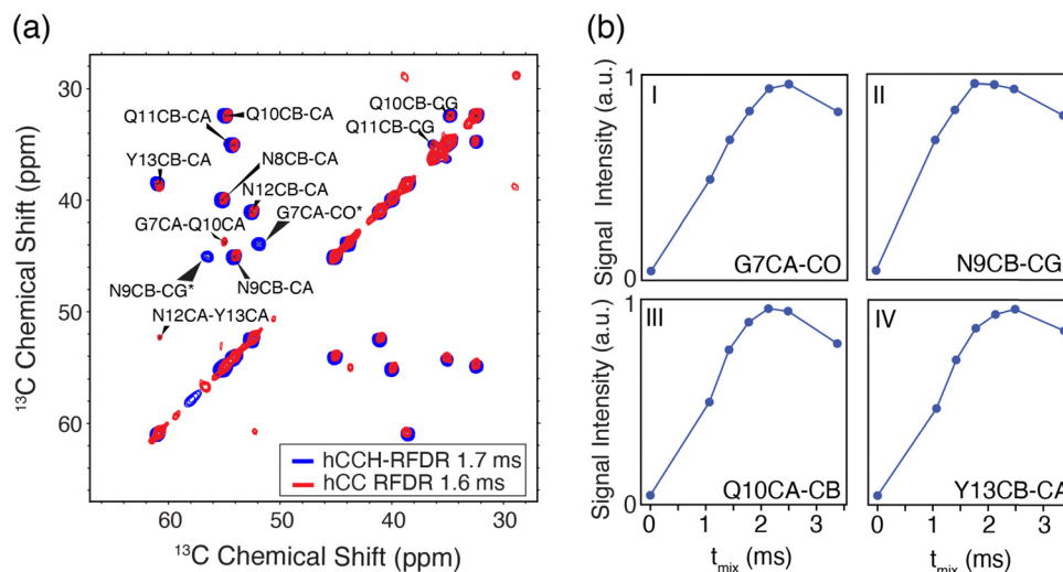
Fig. 3 hCCH-RFDR spectra of nanocrystalline GNNQQNY. (a) The ^{13}\text{C} – ^{13}\text{C} correlations of hCCH-RFDR (red) and hCC RFDR (blue) of [\text{U}\text{-}^{13}\text{C},^{15}\text{N}] -GNNQQNY crystals. The hCCH-RFDR spectrum was acquired at \omega_r/2\pi = 90 kHz using a mixing time of 1.7 ms. The conventional 2-dimensional hCC-RFDR spectrum was acquired at \omega_r/2\pi = 20 kHz MAS using a mixing time of 1.6 ms. The N9CB- \text{C}\gamma^* and G7CA- \text{C}\alpha^* peaks are folded. (b) Signal intensity as a function of RFDR mixing time for hCCH-RFDR. For each contact in I–IV, the normalized signal intensity is plotted.
