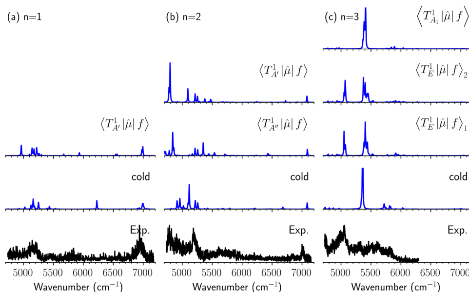
Fig. 8 Comparison among the observed spectrum and simulated cold and hot band spectra of \text{H}_3\text{O}^+\cdots(\text{CO})_n , (a) n = 1 , (b) n = 2 , and (c) n = 3 , in the OH-stretching overtone region. The observed spectra are reproductions of those shown in Fig. 3. In the hot band spectrum simulation, transitions from the first excited level of the OH...CO hydrogen-bond stretching modes ( T_{A'} for n = 1 , T_{A'} and T_{A''} for n = 2 , T_{A_1} and degenerated T_E for n = 3 ) are calculated.
