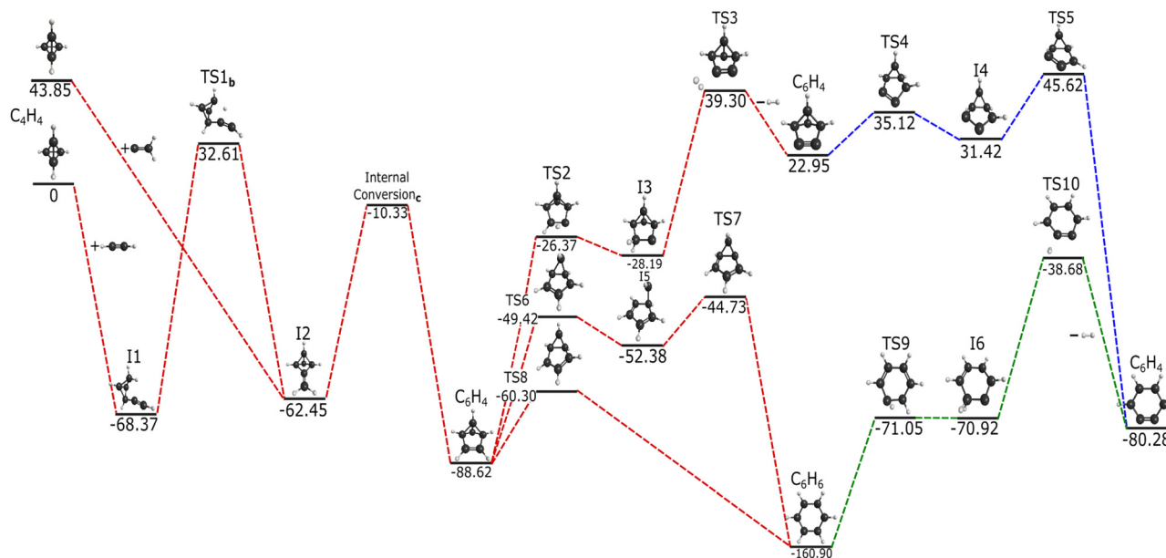
Fig. 5 Reaction pathway for the formation of c\text{-C}_6\text{H}_6 and c\text{-C}_6\text{H}_4 via \text{HC}\equiv\text{CH} and :\text{CCH}_2 addition to c\text{-C}_4\text{H}_4 in kcal mol -1 . TS1 b represents the transition state analyzed in Fig. 6. Internal conversion c represents the intersection seen in Fig. 7. Red dashed lines represent this research, blue dashed lines are based on Poland et al. , 12 and green dashed lines are inspired from Kislov et al. 14
