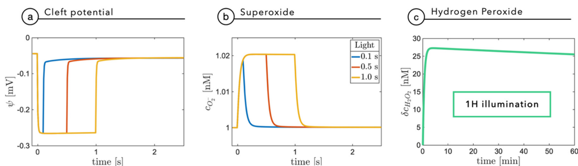
Fig. 6 Panels (a) and (b) show the simulation of the changes in the electric potential \psi(0, t) and the superoxide concentration in response to light stimuli at a power density of 0.2\text{ W m}^{-2} for increasing durations from 100 ms to 1 s. Panel (c) illustrates the variation of the hydrogen peroxide concentration with respect to its equilibrium value after one hour of illumination.
