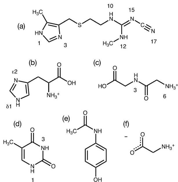
Fig. 1 Structures of the benchmark compounds studied showing nitrogen numbering. The structures evaluated include cimetine (a), histidine HCl H 2 O (b), glycyl glycine HCl H 2 O (c), thymine (d), acetaminophen (e), and zwitterionic glycine (f).
