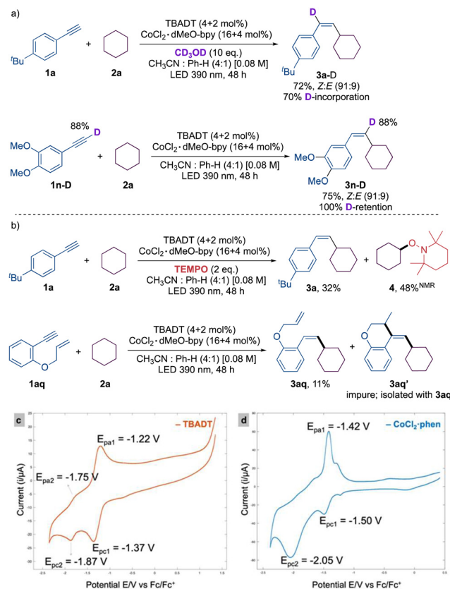
Scheme 2 (a) Deuterium labelling experiments, and (b) radical trap experiments. Cyclic voltammogram of (c) TBADT and (d) \text{CoCl}_2 \cdot 1,10\text{-phenanthroline} .
