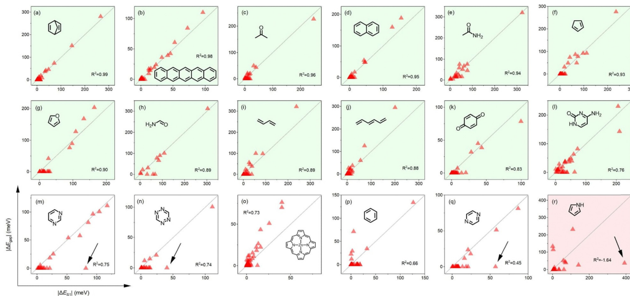
Fig. 1 Electronic-vibrational coupling calculated using \Delta E_{gap} (vertical axis) and \Delta E_{S1} (horizontal axis; both in meV) for selected molecules from Thiel's set, decomposed by normal modes (triangles) and evaluated for zero-point vibrations. Black arrows in (m), (n), (q) and (r) correspond to stretching vibrations with a large \Delta E_{S1} relative to \Delta E_{gap} . Results for remaining molecules are given in Fig. S1 (ESI†).
