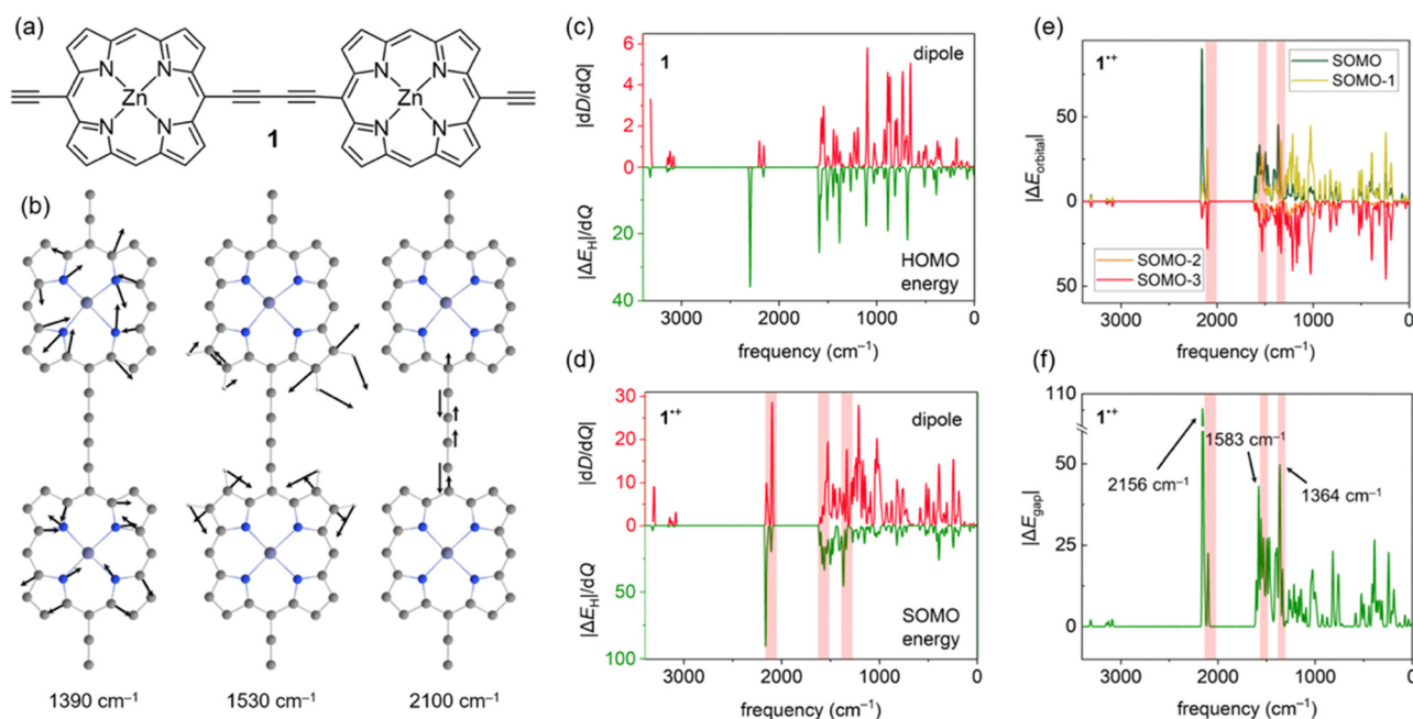
Fig. 2 (a) Structure of \mathbf{1} . (b) Calculated IRAVs of \mathbf{1}^{+\bullet} . (c)–(d) Coupling between the computed IR intensities (positive y axis) and derivatives of frontier orbital energies (negative y axis) in (c) \mathbf{1} and (d) \mathbf{1}^{+\bullet} . Note the different y scales. (e) Contribution of lower-lying orbitals of \mathbf{1}^{+\bullet} . (f) Modulation of the fundamental gap \Delta E_{\text{gap}}/dQ_i in \mathbf{1}^{+\bullet} with molecular vibrations.
