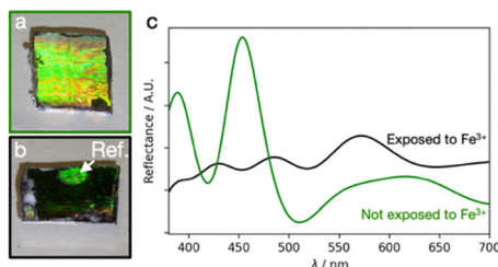
Fig. 4 Colorimetric detection of \text{Fe}^{3+} ions from aqueous solutions. (a) Photograph of a Schiff base-functionalized IO exposed to a 20% ethanolic aqueous solution without previous exposure to \text{Fe}^{3+} . The structural coloration is clearly observed as the sample is not wetted by the liquid. (b) An IO with the identical surface chemistry exposed to a 20% ethanolic solution previously exposed to a 60% EtOH \text{Fe}^{3+} solution is wetted and does not exhibit structural color. Note the colored spot on the top of the sample – indicated by the white arrow – was not exposed to \text{Fe}^{3+} by protecting it with an epoxy resin and served as an internal reference. The photographs were collected at a slight angle to emphasize the color. (c) Corresponding reflectance spectra of both samples, showing the suppression of the photonic stop band upon exposure to \text{Fe}^{3+} ions.
