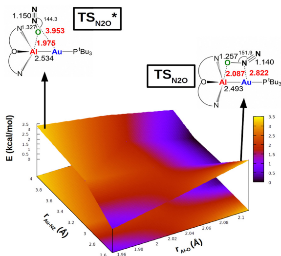
Fig. 6 Potential energy surface (PES) in the region neighbouring the transition state TS for the reaction of complex [ t Bu 3 PAuAl(NON)] with N 2 O. Insets: Position on the PES and schematic structure of TS and TS*. Energy has been shifted in each case according to the minimum energy structure. Reproduced with permission from ref. 63 Copyright 2023, Wiley-VCH GmbH.
