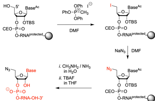
Fig. 4 Solid-phase synthesis of 5'-azido modified oligoribonucleotides. Reagents and conditions: (i) 0.5 M MTPI/DMF, rt, 1 h; (2) sat. \text{NaN}_3 solution in DMF, 55 °C, 5 h; (3) (i) 40% aq \text{MeNH}_2 /30% aq \text{NH}_3 (1/1 v/v), 40 °C, 4 h, (ii) 1 M TBAF/THF, 37 °C, 16 h.
